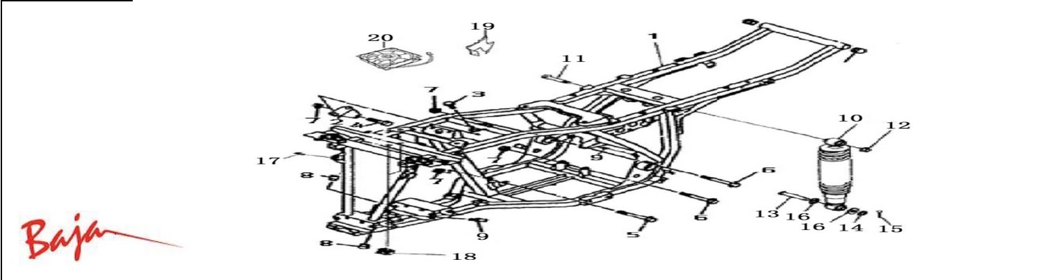
FIG. 16 FRAME, REAR SHOCK
