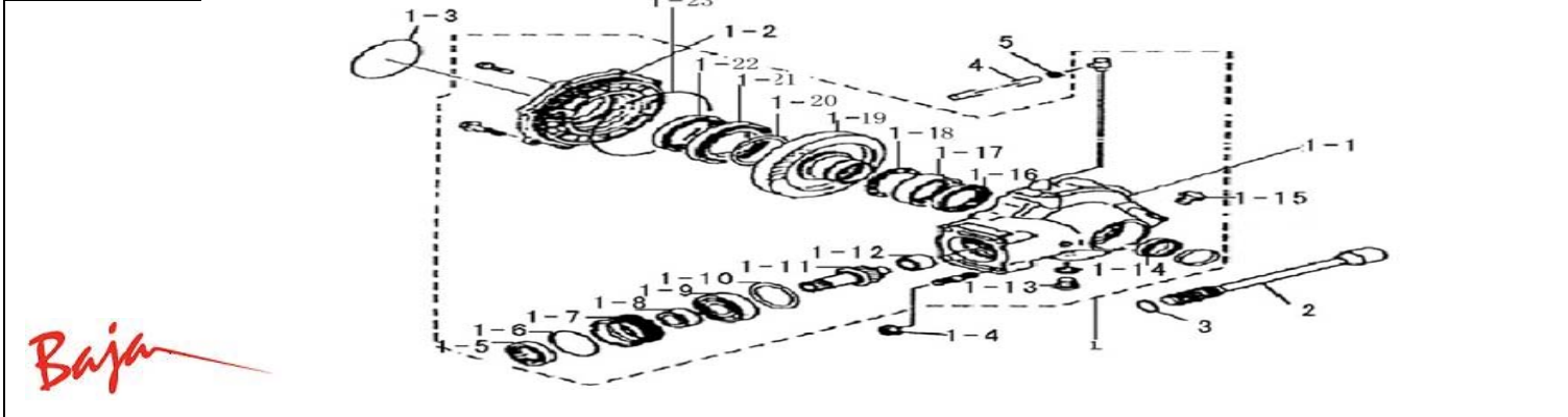
FIG. 23 REAR DRIVING GEAR BOX
